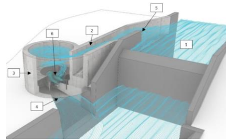
Fig. 2. Parts of a gravitational vortex turbine. Source: Velásquez, L., Chica, E. and Posada, J. [4]
