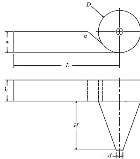
Fig. 3. Geometric parameters of the GVHT.
