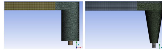
Fig. 8. Geometric configurations of inlet channel and vortex formation in terms of flow.
