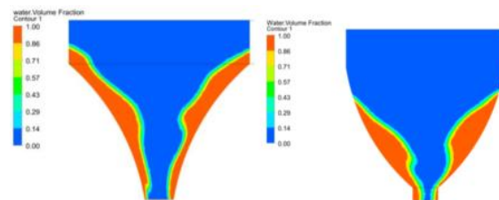
Fig. 9. Conical basins with concave and convex cross-sections.
