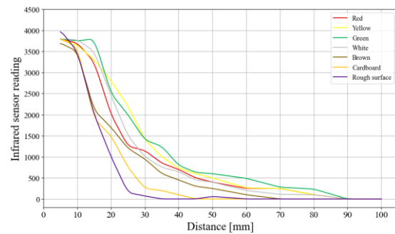
Fig. 3. Infrared Sensor Range.
