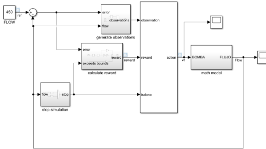
Fig. 6. Block diagram of the learning environment
