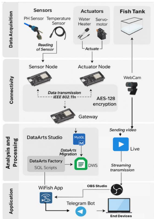
Fig. 1. System architecture. Source: Authors.
