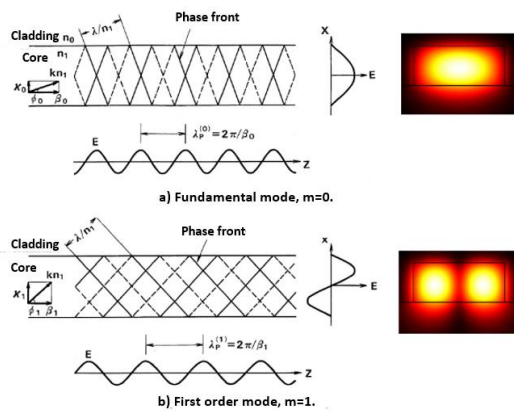
Fig. 2. Formation of Propagation Modes. (a) Fundamental Mode (b) First Order Mode Source: adapted from [19]
