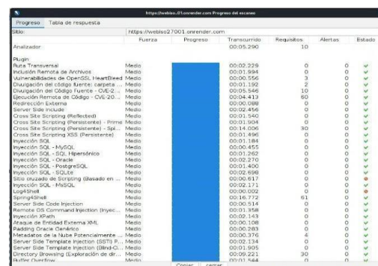
Fig. 8. Results of spidering attack - Front-end. Source: Owasp-zap.
