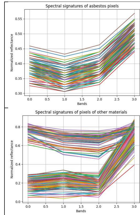
Fig. 3. Spectral signatures of the 4-band pixels. Source: own elaboration.
