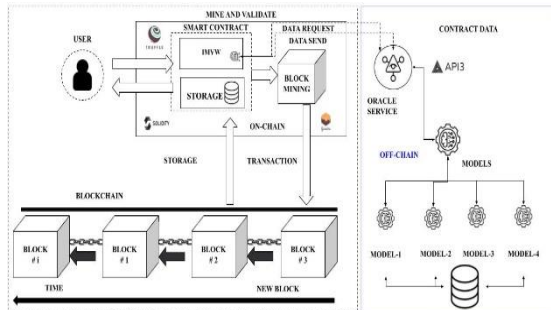
Fig. 1. Proposed blockchain oracle architecture. Source: Authors.
