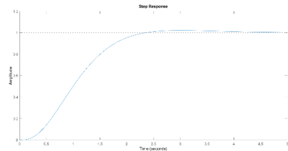
Fig. 9. RVE controller response by pole placement. Source: own elaboration.
