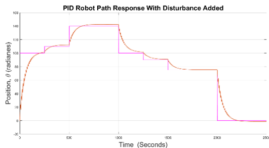
Fig. 11. PID control response with disturbance added. Source: own elaboration.
