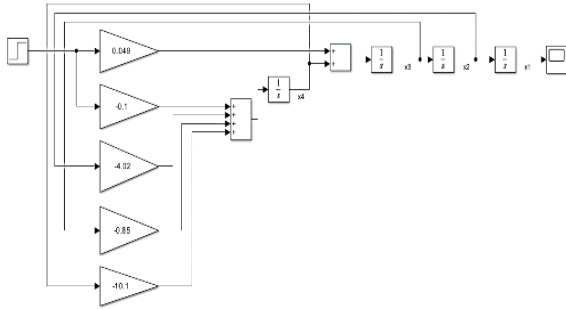
Fig. 6. SEA Model Representation of State by Equations. Source: own elaboration.
