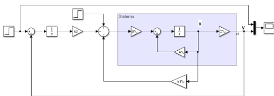
Fig. 12. State Observer. Source: own elaboration.
