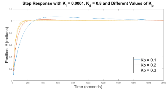
Fig. 8. SEA PID tuning. Source: own elaboration.
