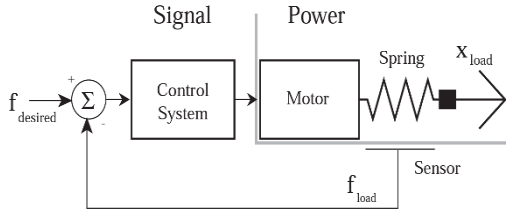
Fig. 1. SEA actuator components. Source: own elaboration.
