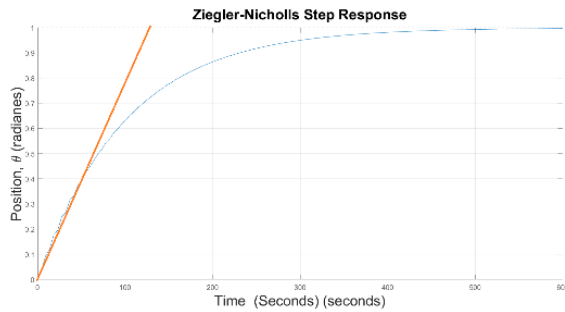
Fig. 7. SEA PID reaction curve. Source: own elaboration.
