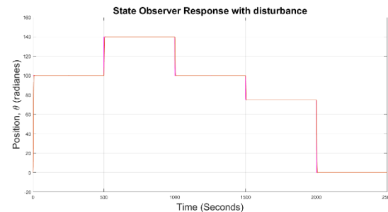
Fig. 13. SEA State observer response Source: own elaboration.
