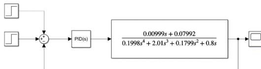
Fig. 10. PID with added disturbance. Source: own elaboration.
