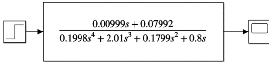
Fig. 4. Final Model of SEA with Parameters. Source: own elaboration.
