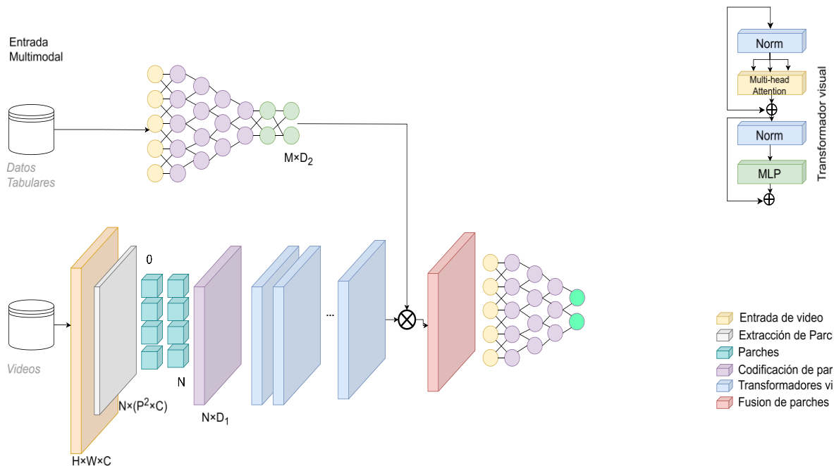
Fig. 3. Architecture Design for a binary classification model based on Multimodal Deep Learning ViT.
