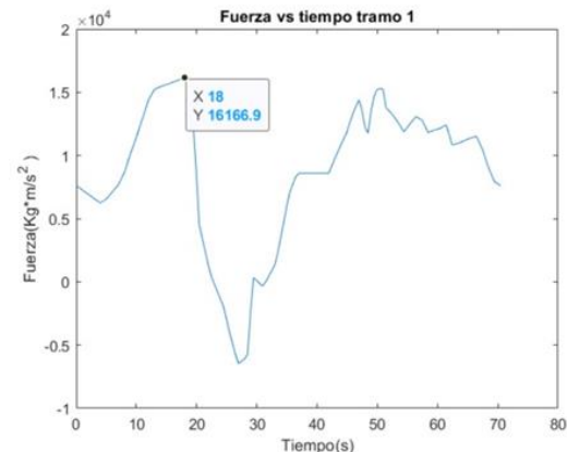
Fig. 11. Highest force obtained pre-selected route. Section 1
