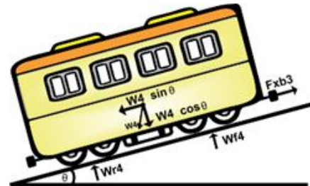
Fig. 5. Free body diagram wagon 4 (Trailer)
