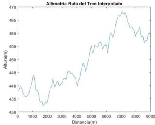
Fig. 9. Altimetry of the preselected route for the metro line.
