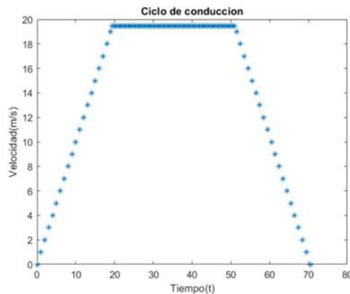
Fig. 10. Driving cycle
