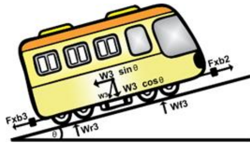
Fig. 4. Free body diagram wagon 3(traction)
