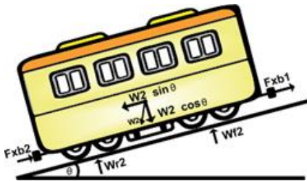
Fig. 3. Free body diagram wagon 2 (Trailer)
