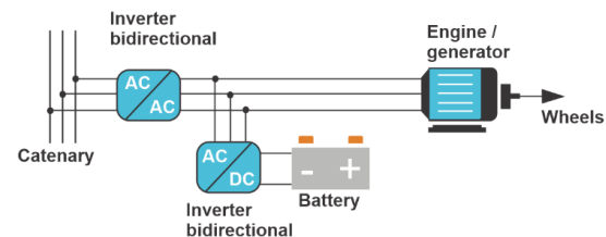
Fig. 8. Bi-directional inverter topology driving the AC motor
