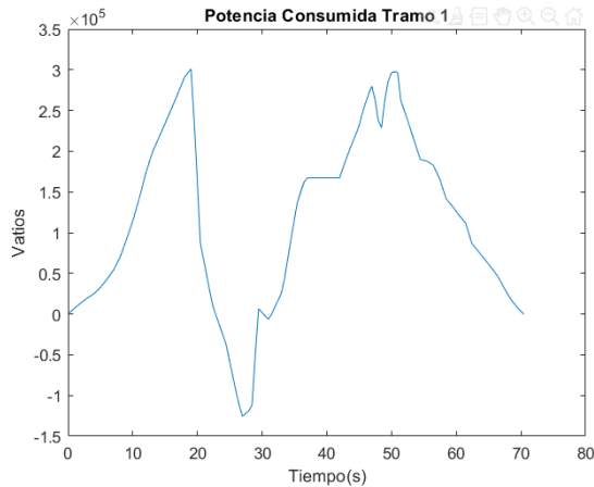
Fig. 13. Section with the highest power consumption on the road. Section 1
