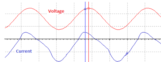
Fig. 1. Voltage and current characteristics at the input of a single-phase rectifier with an inductive load and no PF correction. Source: own elaboration.
