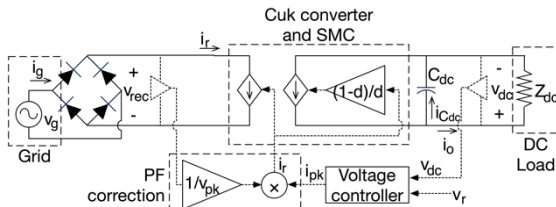
Fig. 3. Rectifier considering the action of the SMC and the PF correction strategy.
