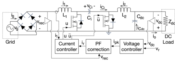
Fig. 2. Rectifier based on the Cuk converter with voltage regulation and PF correction.
