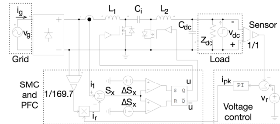
Fig. 4. Electrical scheme for the detailed simulation in PSIM.
