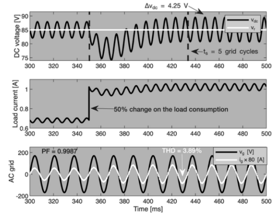
Fig. 6. Detailed simulation of the Cuk rectifier for Case 2 (buck mode, v_{dc} = 85 V). Source: own elaboration.
