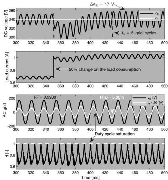
Fig. 7. Detailed simulation of the Cuk rectifier for Case 1 with a PI current controller.
