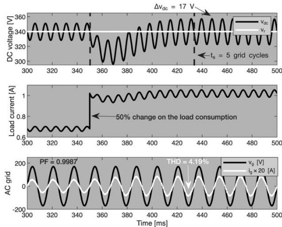
Fig. 5. Detailed simulation of the Cuk rectifier for Case 1 (boost mode, v_{dc} = 340 V). Source: own elaboration.
