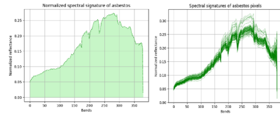
Fig. 3. Characteristic spectral signature of asbestos-cement.
