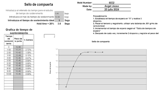
Fig. 3. Damper seal test. Source: own elaboration
