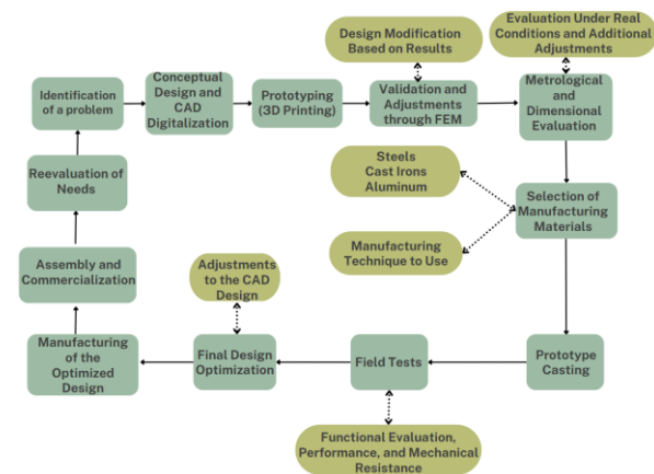
Fig. 1. Design methodology CAD/CAM/CAE for the design and manufacturing of a manual agricultural tool. Adapted from [14]
