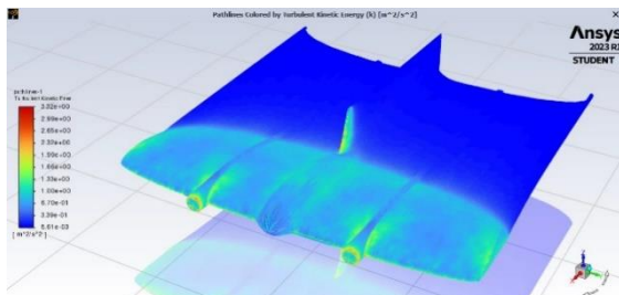
Fig. 13. Turbulent kinetic energy at 0^\circ AoA Source: own elaboration
