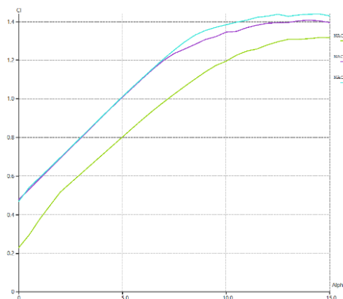
Fig. 2. Relationship between the lift coefficient C_L with attack angle Alpha for the three proposed airfoils Source: own elaboration
