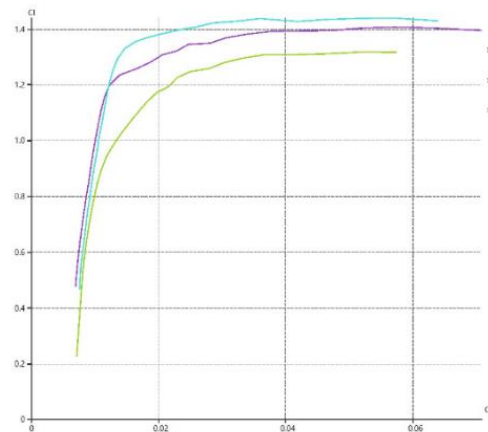
Fig. 3. Relationship between the lift coefficient C_L and drag coefficient C_d for the three proposed airfoils.
