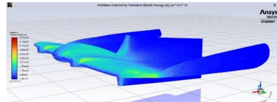
Fig. 15. Turbulent kinetic energy at 10^\circ AoA Source: own elaboration
