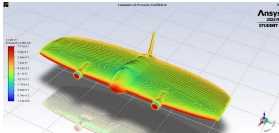
Fig. 12. Contours of pressure coefficient at 0^\circ AoA Source: own elaboration
