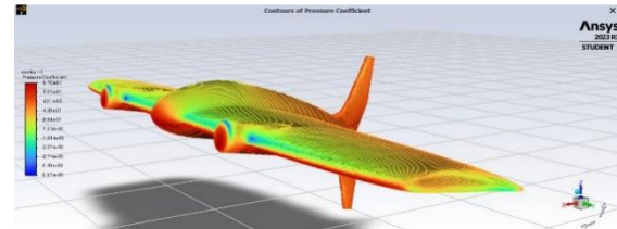
Fig. 14. Contours of pressure coefficient at 10^\circ AoA Source: own elaboration
