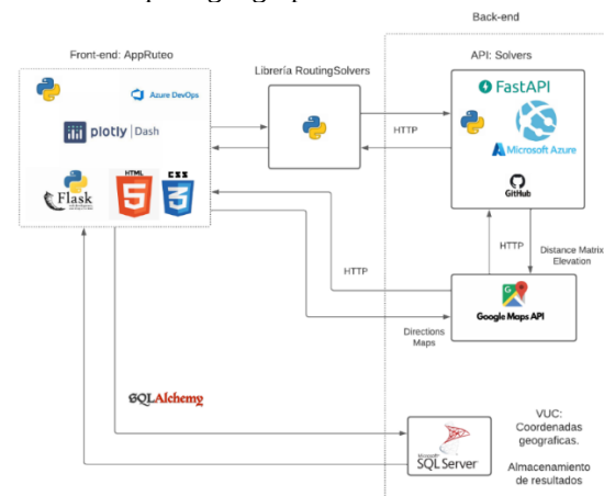
Fig. 3. Implementation Architecture
