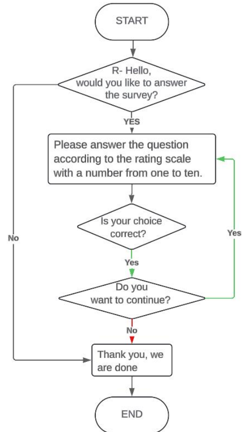
Fig 1. Summary dialogue model
