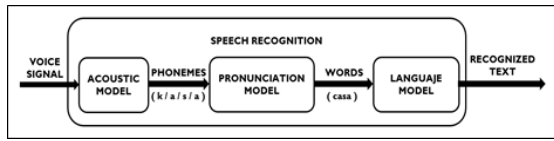
Fig. 2. Block diagram of speech recognition. Source: own elaboration.
