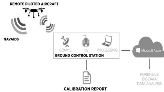
Fig. 5 Canard UAS architecture.
