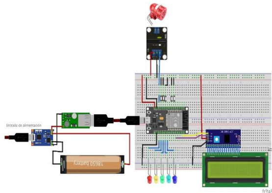
Fig 3. Connection diagram of the electronic circuit.
