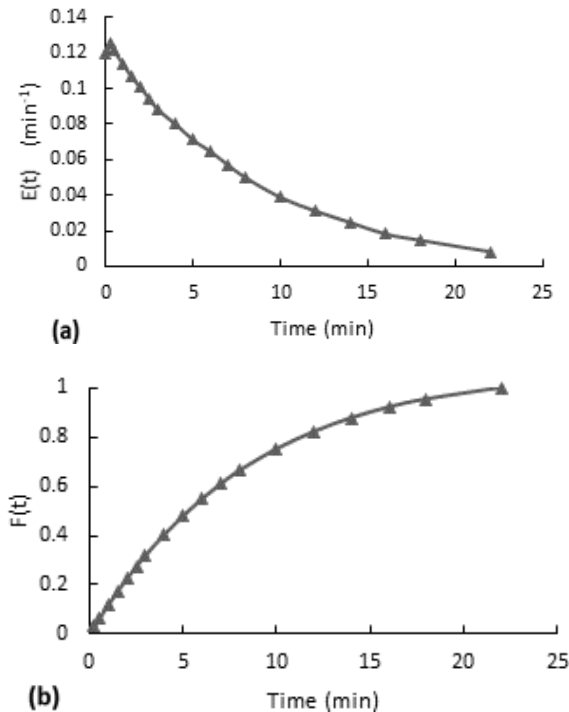
Fig. 8. Residence time distribution curves for the stirred experiment with the packaging mesh and minimum flow. (a) E(t) curve, (b) accumulative distribution function F(t)
