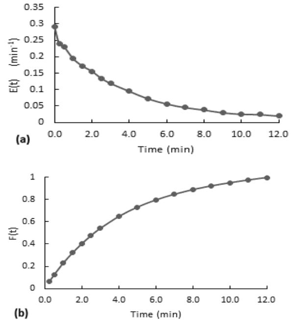
Fig. 9. Residence time distribution curves for the stirred experiment with the packaging mesh and minimum flow. (a) E(t) curve, (b) accumulative distribution function F(t)
