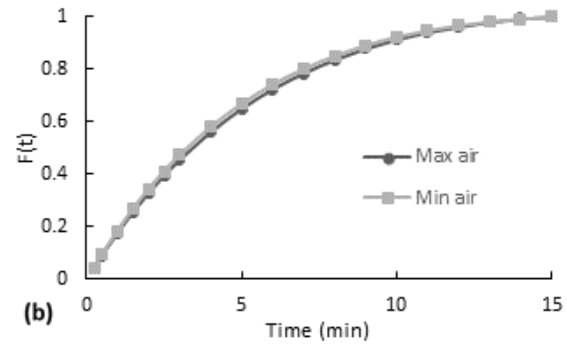
Fig. 7. Residence time distribution curves for the stirred experiment without the packaging mesh. (a) E(t) curve, (b) accumulative distribution function F(t)
