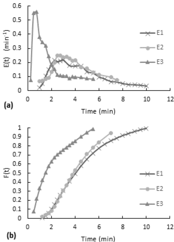
Fig. 6. Residence time distribution curves for the maximum flow, with packaging and no stirring experiment. (a) E(t) curve, (b) accumulative distribution function F(t)
