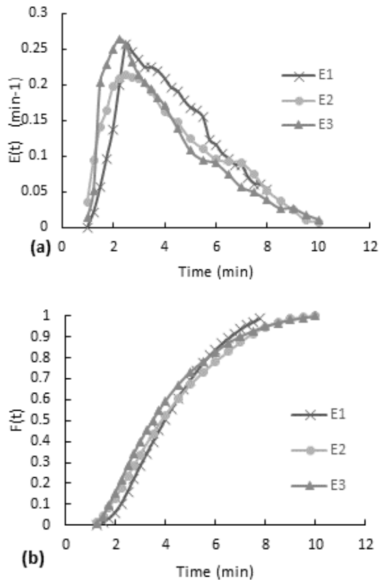
Fig. 4. Residence time distribution curves for the maximum flow, no packaging, and no stirring experiment. (a) E(t) curve, (b) accumulative distribution function F(t) .
