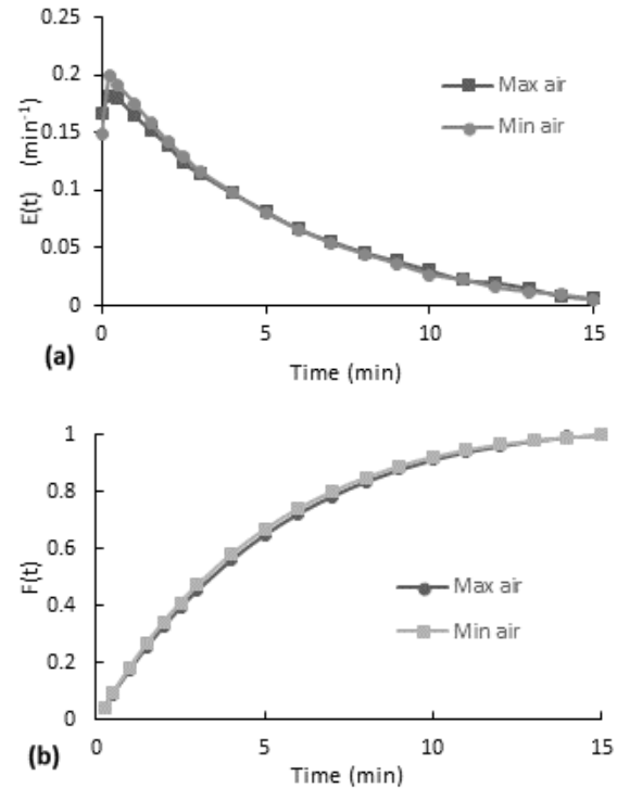
Figure 7. Residence time distribution curves for the stirred experiment without the packaging mesh. (a) E(t) curve, (b) accumulative distribution function F(t)
