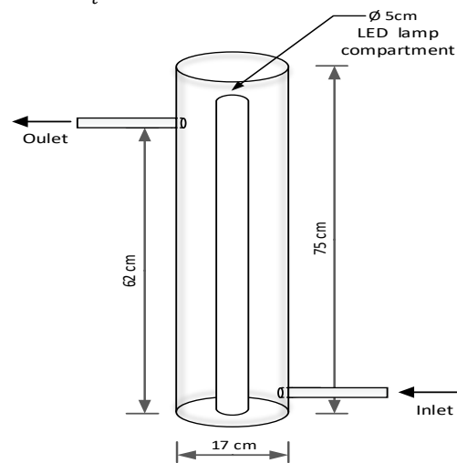
Figure 1. Schematic diagram of the annular catalytic reactor.
