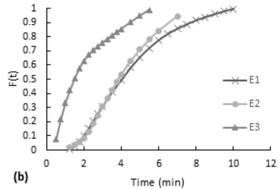
Figure 6. Residence time distribution curves for the maximum flow, with packaging and no stirring experiment. (a) E(t) curve, (b) accumulative distribution function F(t)
