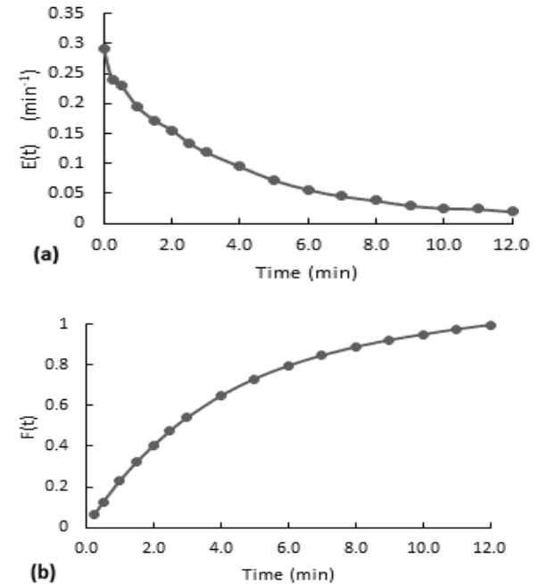
Figure 9. Residence time distribution curves for the stirred experiment with the packaging mesh and minimum flow. (a) E(t) curve, (b) accumulative distribution function F(t)
