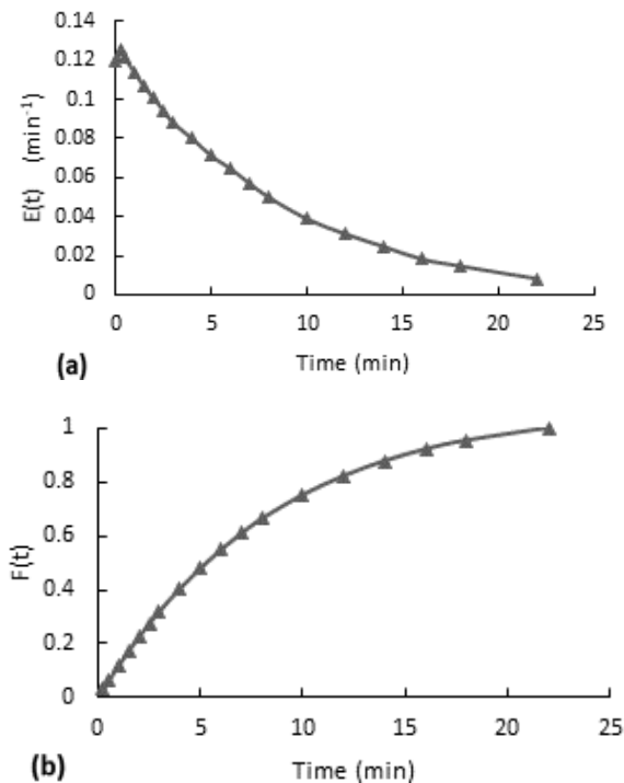
Figure 8. Residence time distribution curves for the stirred experiment with the packaging mesh and minimum flow. (a) E(t) curve, (b) accumulative distribution function F(t)
