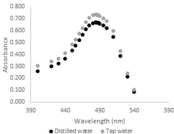
Figure 2. Absorbance at different wavelengths for dye solutions (Orange II), with distilled water and tap water.
