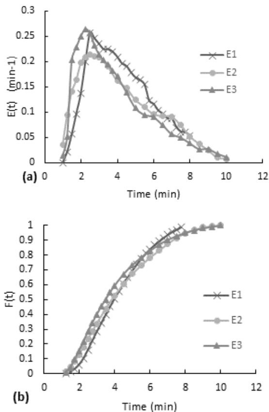
Fig. 4. Residence time distribution curves for the maximum flow, no packaging, and no stirring experiment. (a) E(t) curve, (b) accumulative distribution function F(t) .
