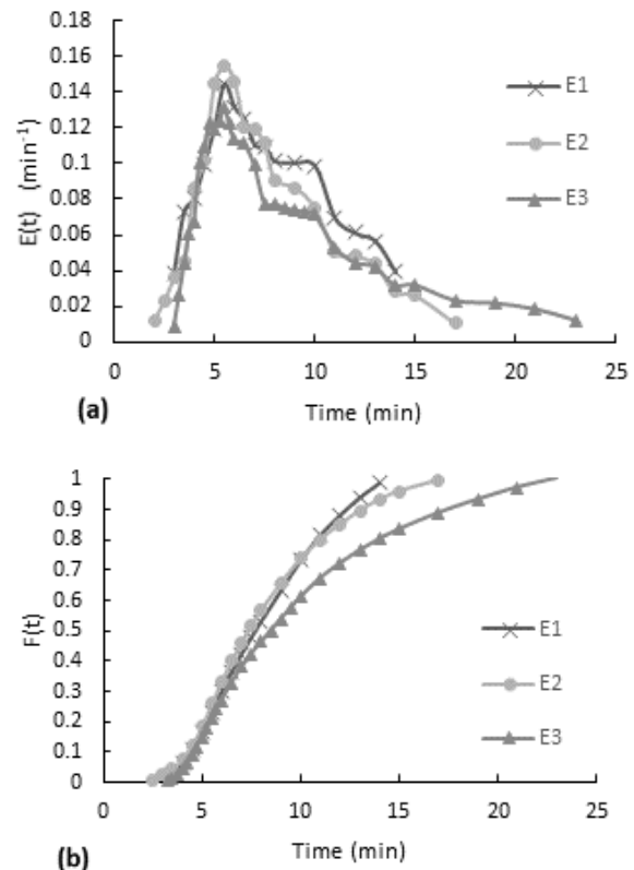
Fig. 3. Residence time distribution curves for the minimum flow, no packaging, and no stirring experiment. (a) E(t) curve, (b) accumulative distribution function F(t) .
