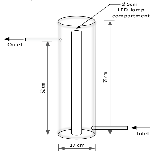
Fig. 1. Schematic diagram of the annular catalytic reactor.
