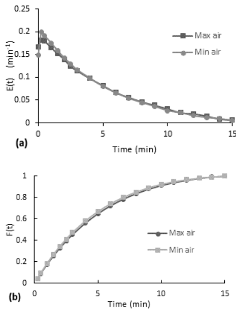
Fig. 7. Residence time distribution curves for the stirred experiment without the packaging mesh. (a) E(t) curve, (b) accumulative distribution function F(t)
