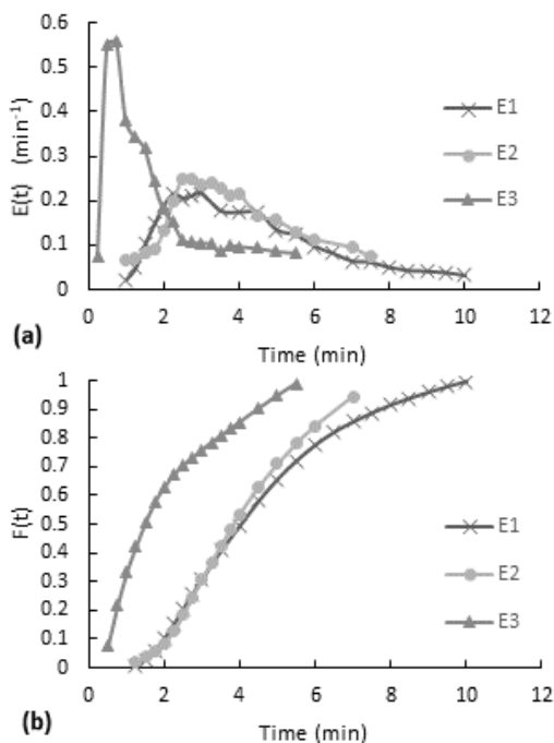
Fig. 6. Residence time distribution curves for the maximum flow, with packaging and no stirring experiment. (a) E(t) curve, (b) accumulative distribution function F(t)
