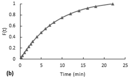
(b) Fig. 8. Residence time distribution curves for the stirred experiment with the packaging mesh and minimum flow. (a) E(t) curve, (b) accumulative distribution function F(t)
