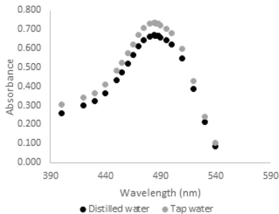
Fig. 2. Absorbance at different wavelengths for dye solutions (Orange II), with distilled water and tap water.
