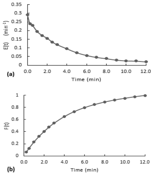
(a) (b) Fig. 9. Residence time distribution curves for the stirred experiment with the packaging mesh and minimum flow. (a) E(t) curve, (b) accumulative distribution function F(t)
