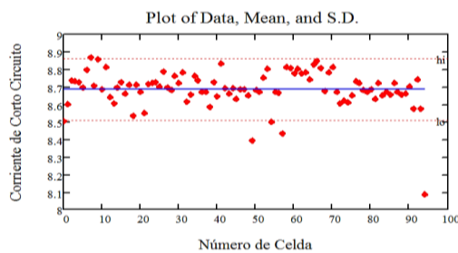
Fig. 7 Graphic Representation of the Short Circuit Current Measurements with their Respective Average Value and Errors
