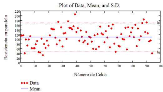
Fig. 13 Graphic Representation of Resistance Measurements in Parallel with their Respective Mean Value and Errors
