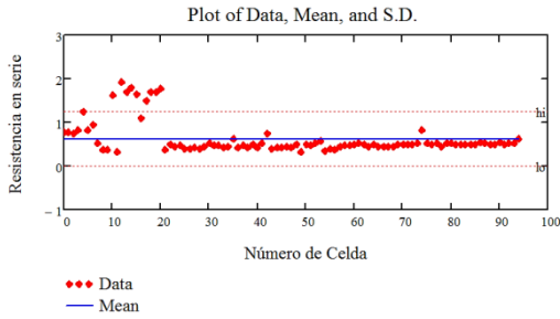
Fig. 12 Graphic Representation of the Resistance Measurements in Series with their Respective Average Value and Errors
