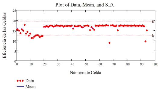
Fig. 14 Graphic Representation of the Efficiency of the Cells, in %, with their Respective Average Value and Errors
