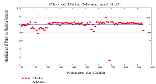
Fig. 10 Graphic Representation of the Measurements of the Intensity at the Point of Maximum Power with its Respective Average Value and Errors
