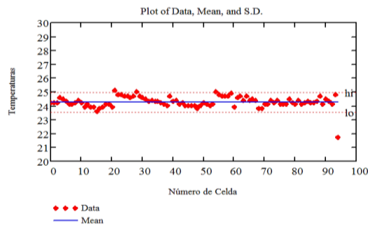
Fig. 5 Graphic Representation of the Temperature Measurements, with their Respective Average Value and Errors
