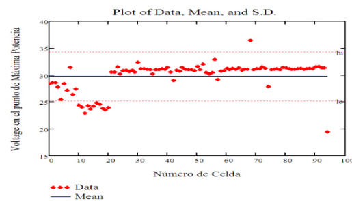
Fig. 9 Graphic Representation of the Measurements of the Voltage at the Point of Maximum Power with its Respective Mean Value and Errors
