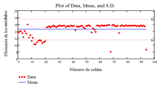
Fig. 15 Graphic Representation of the Efficiency of the Modules, in %, with their Respective Average Value and Errors
