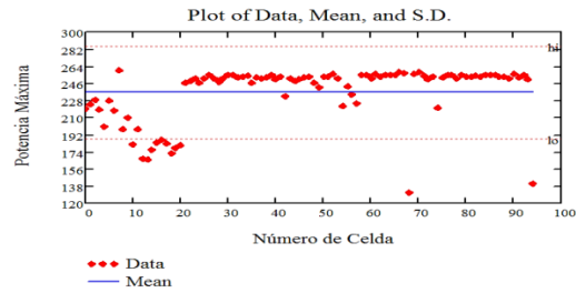
Fig. 8 Graphic Representation of the Maximum Power Measurements with their Respective Average Value and Errors
