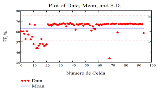
Fig. 11 Graphic Representation of the Filling Factor Measurements with their Respective Mean Value and Errors
