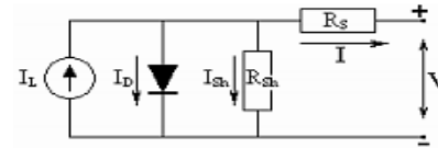
Fig. 1 Equivalent Circuit of a Photovoltaic Solar Cell, by Díaz, 2018
