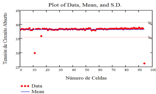
Fig. 6 Graphic Representation of the Open Circuit Voltage Measurements with their Respective Average Value and Errors
