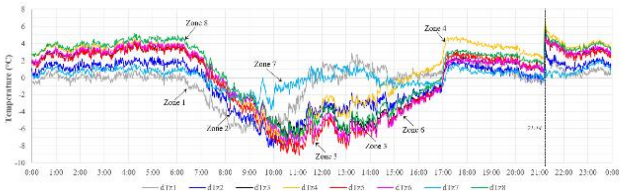
Fig. 13. Variation on soil temperature concerning ambient temperature.
