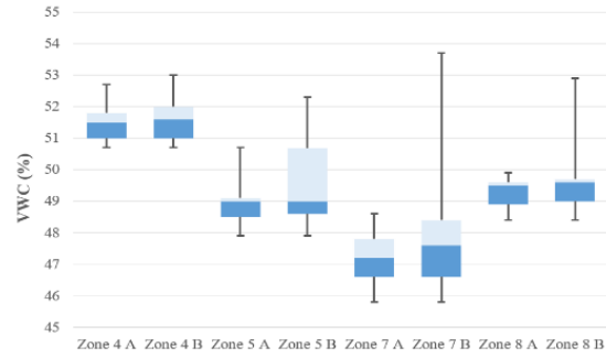
Fig. 10. Boxplots of the soil moisture for zones 4, 5, 7, and 8 with and without the effect of the rainfall during one day.
