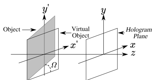
Figure 1: Diffraction between tilted planes
