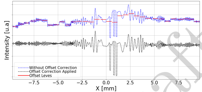
Figure 8: Correction of a profile of the reconstruction plane, before and after applying the Offset .
