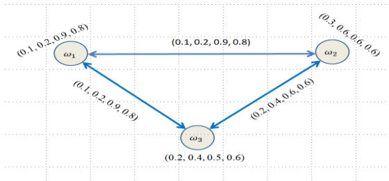
Figure 3: SVQN-graph of Adjacent Vertices
