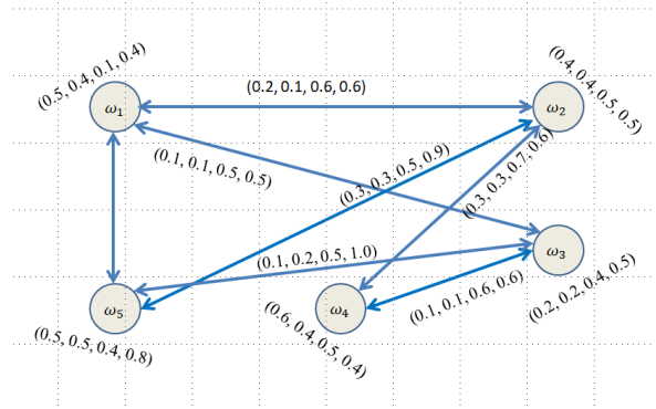
Figure 7: Bipartite SVQN-graph
