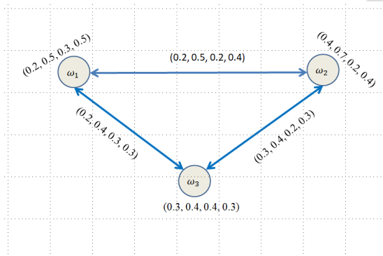
Figure 6: Complete SVQN-graph
