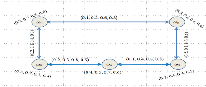
Figure 1: SVQN-graph
